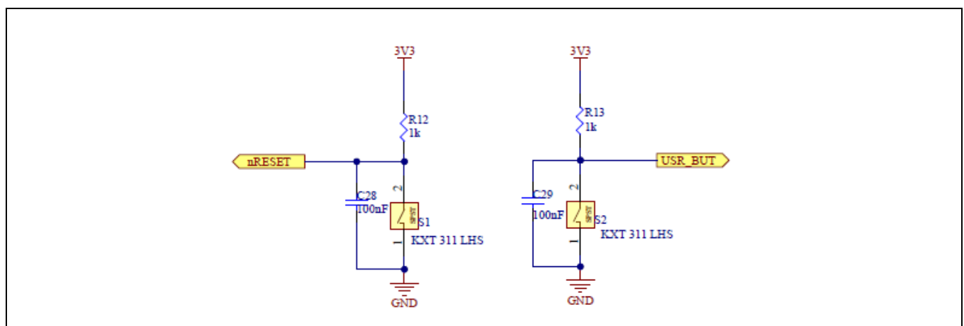
Figure 9 Reset (S1) and user button (S2) schematic
