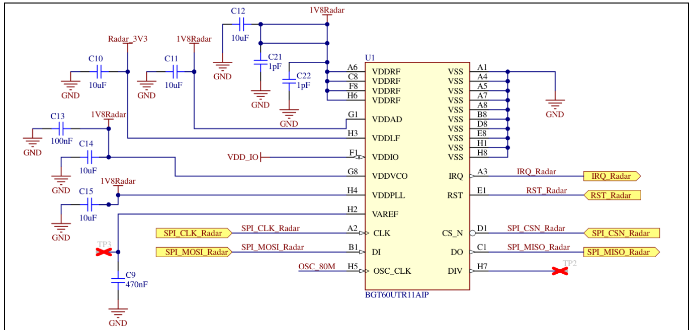
Figure 7 XENSIV™ BGT60UTR11AIP Radar MMIC schematic
