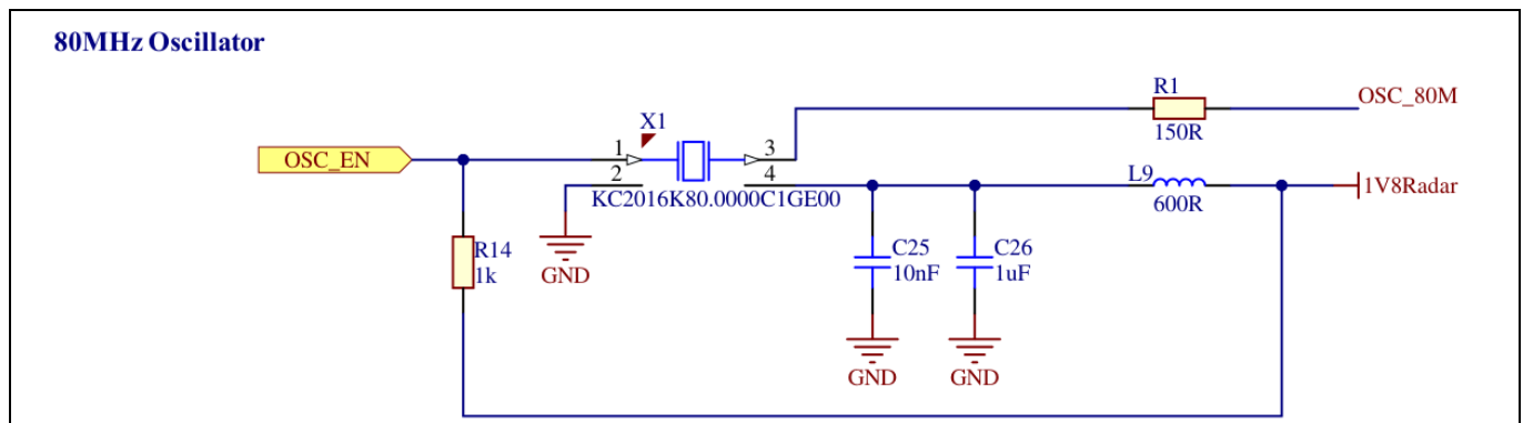
Figure 8 Oscillator circuit on the XENSIV™ BGT60UTR11AIP Wing board
