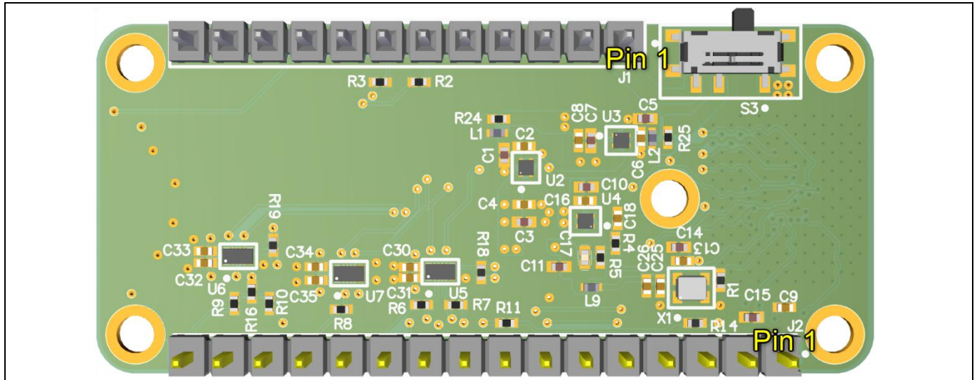
Figure 15 Adafruit headers and test points on bottom of the XENSIV™ BGT60UTR11AIP Radar Wing board
