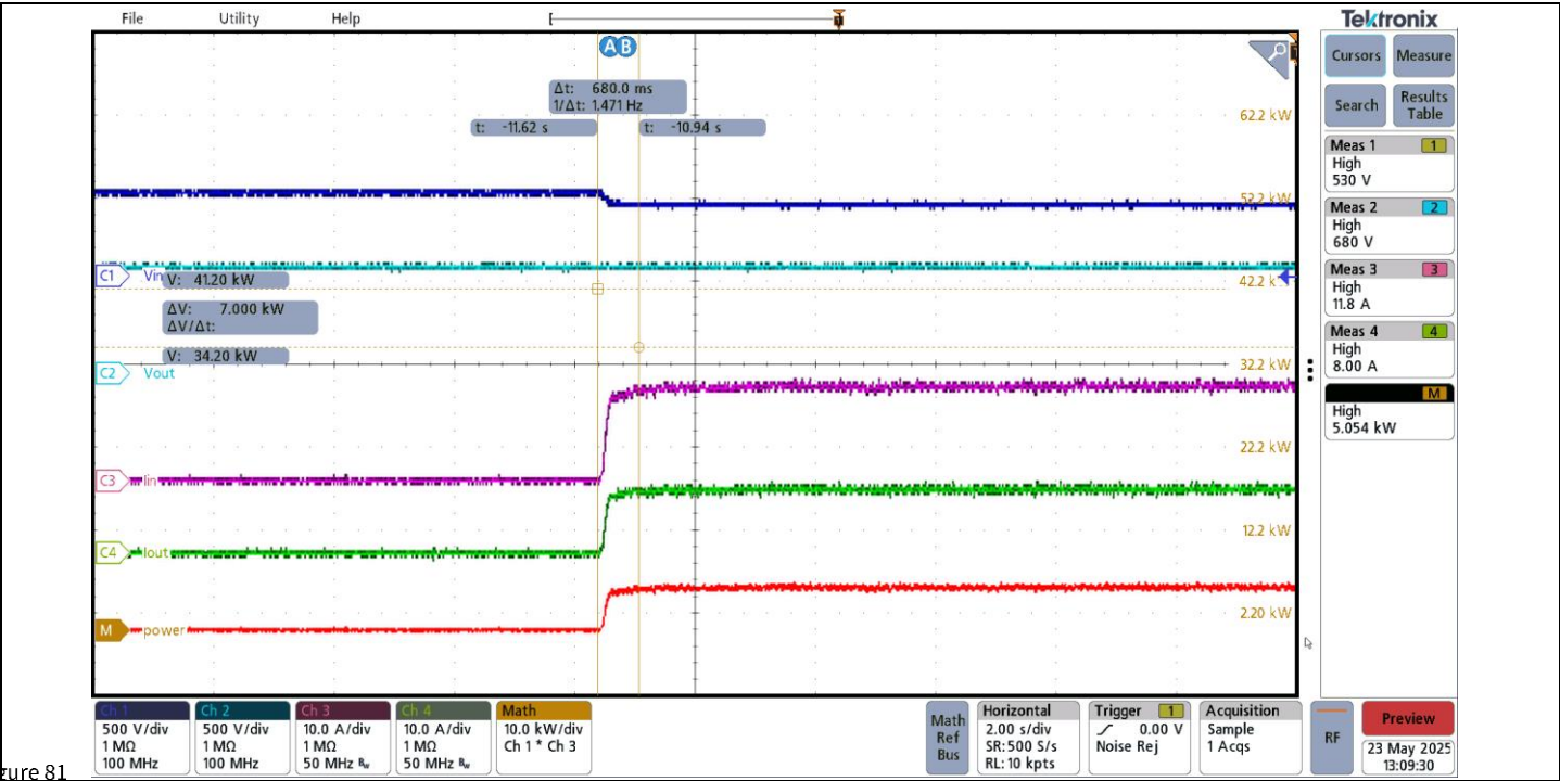
650 V output voltage, 1000 W/m 2 light intensity, 25°C
