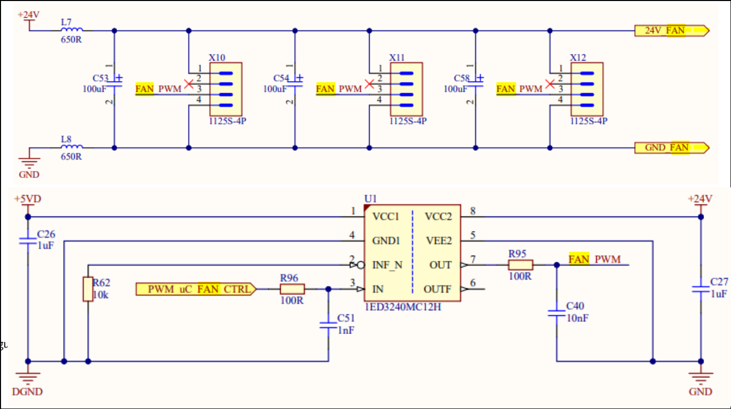
Figure 31 A fan comes with the power board. The fan's duty cycle can be controlled by the GUI and ambient temperature.
