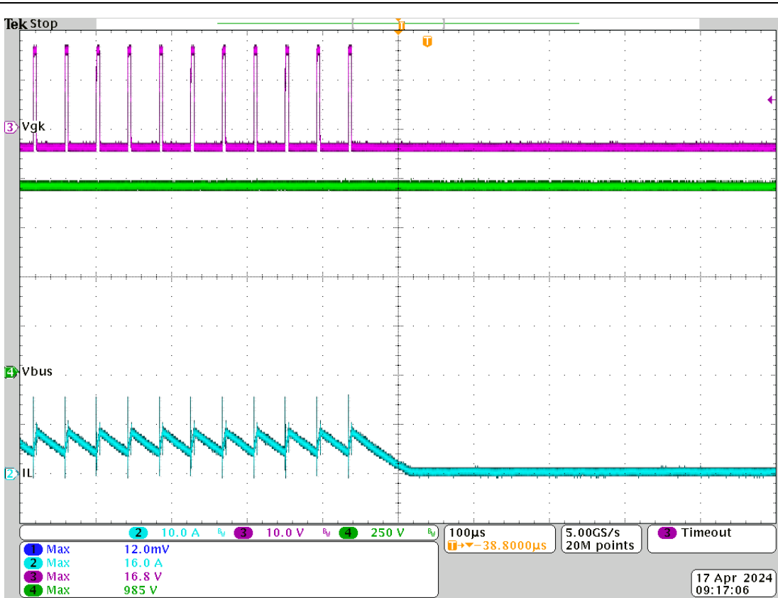
DC-link OVP for channel 1
