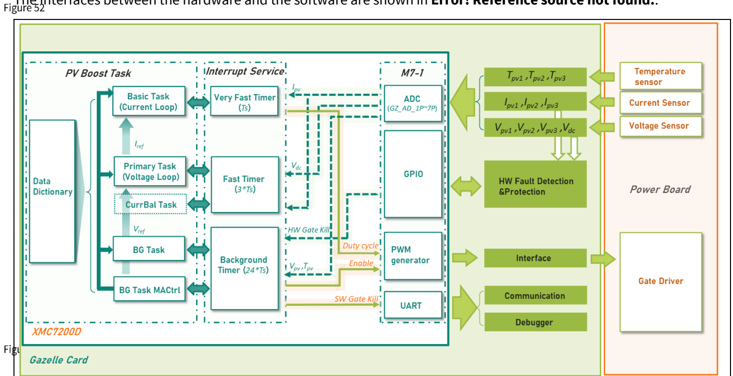
The interfaces between hardware and software ( T_s = 1/24000s )
