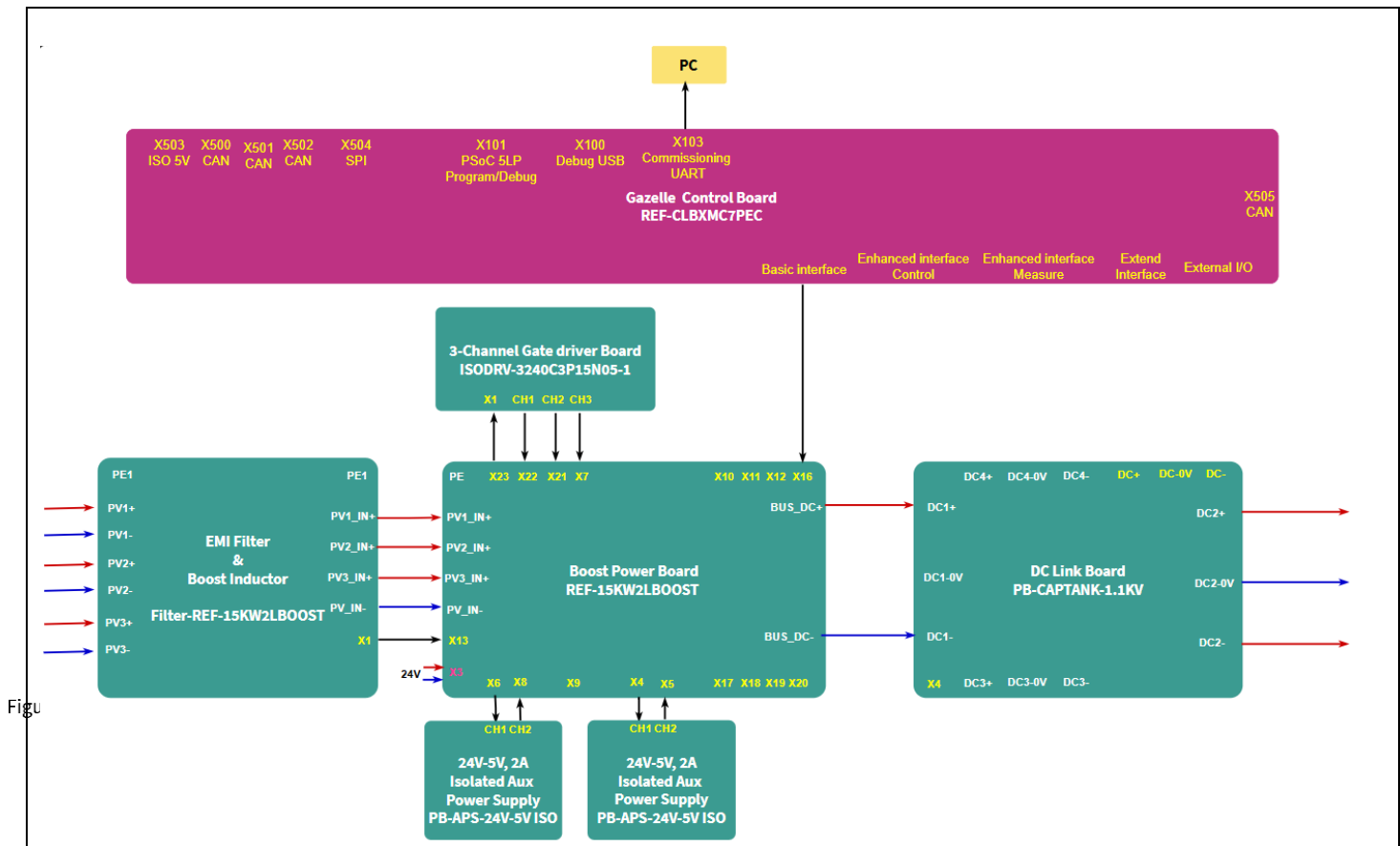
Assembly diagram
